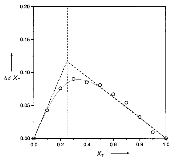
Figure 3. Job plot corresponding to the chemical shift displacement of C-1 of \beta -CD for the 1/3 T /2NS complex. Total concentration [\mathbf{T}] + [2\text{NS}] = 5 \text{ mM} .
