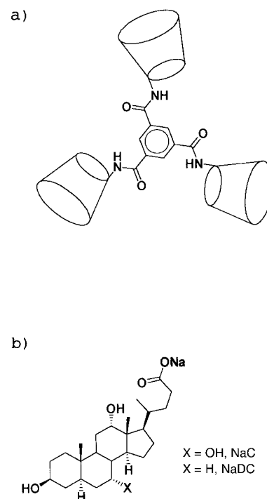
Figure 2. Structures of T (a) and the bile salts NaC and NaDC (b).
