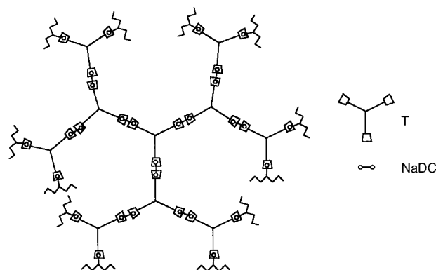
Figure 1. Schematic representation of the Cayley tree dendrimerlike supramolecular structure expected for the cyclodextrin complex T /NaDC.
